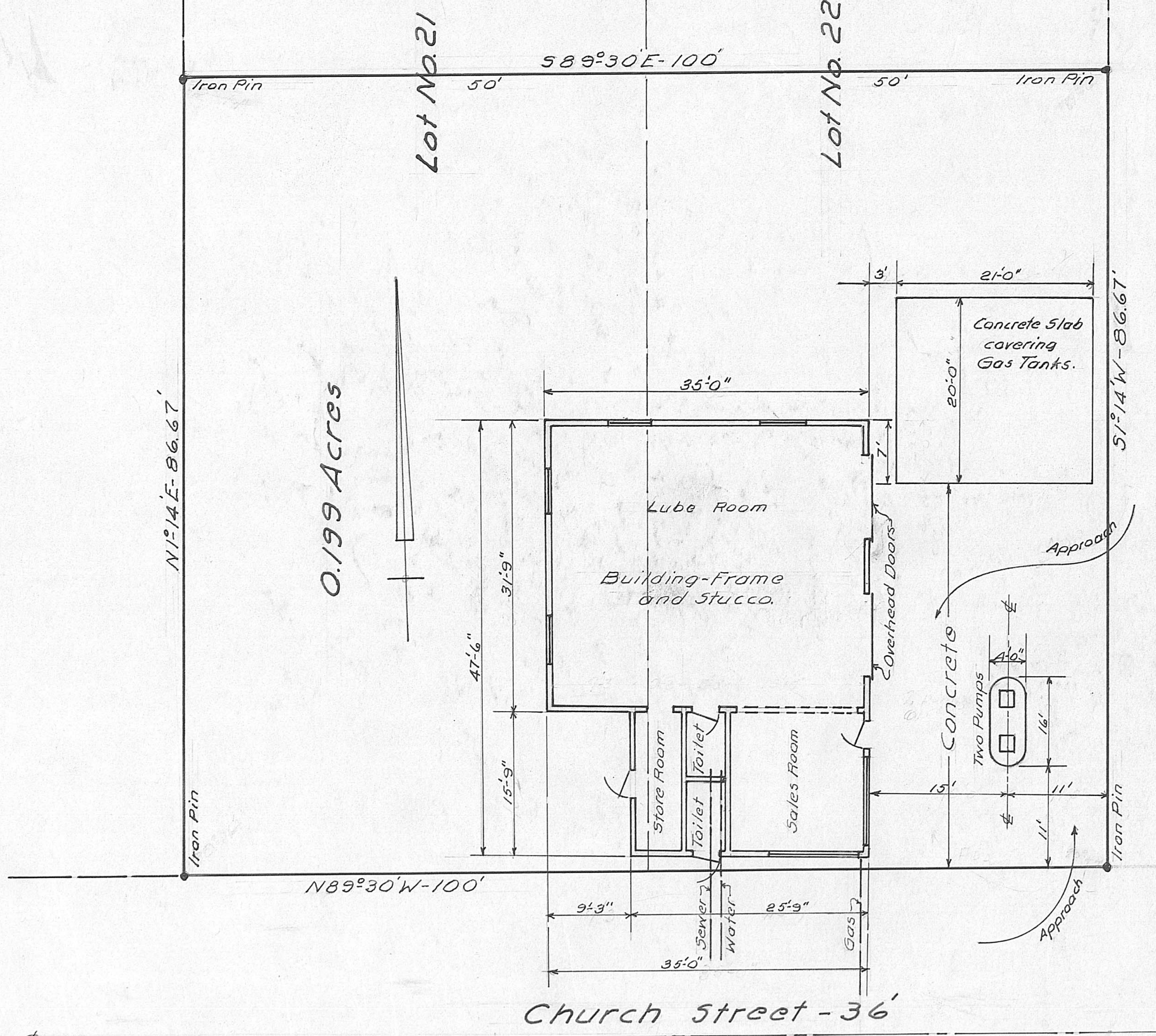
Site Plat of Premises belonging to Dana M. Daniels et al South Solon, Ohio. - 1955
