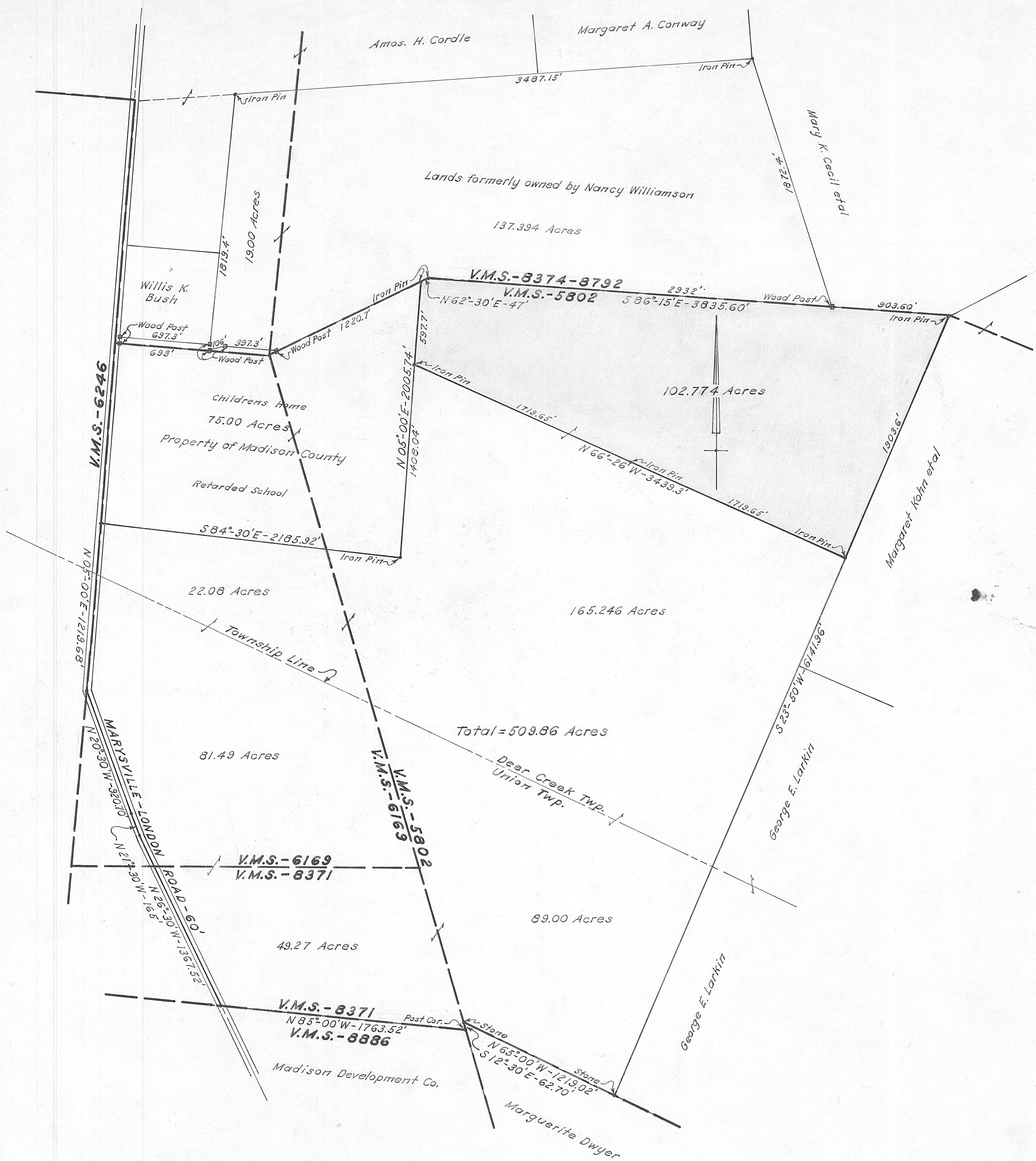
Tract of land in Deer Creek Township, Madison County, Ohio, surveyed for Clinton G. Stickel et al - 1966
