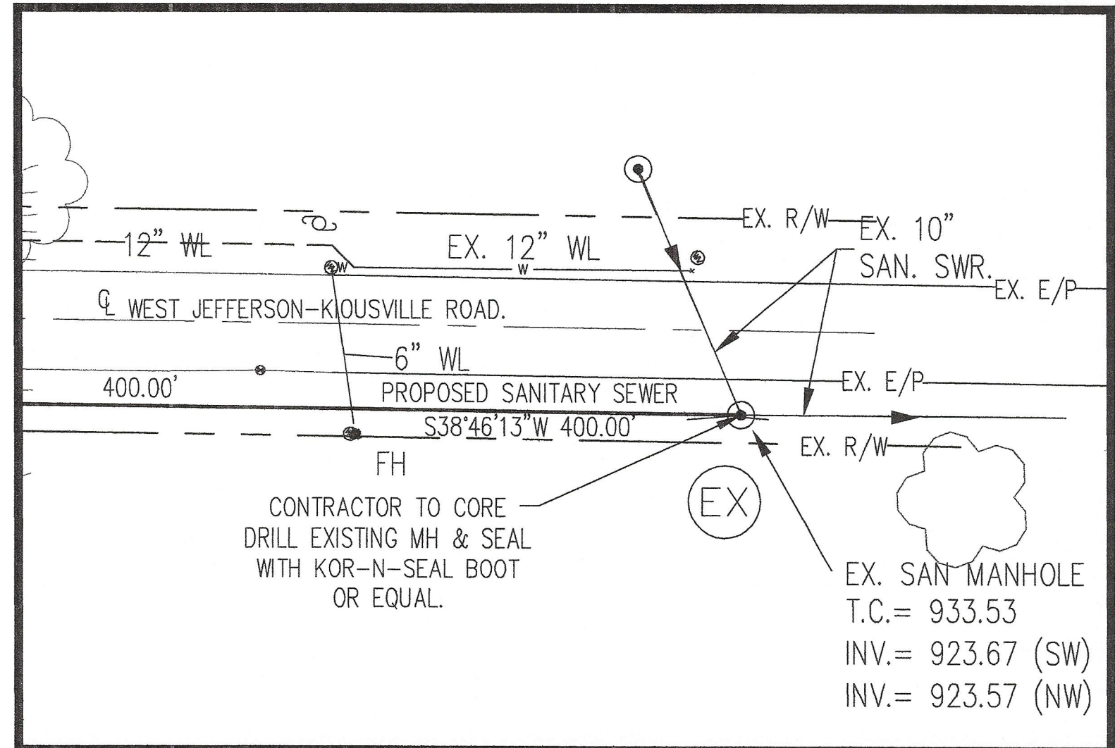
SEWER CONNECTION POINT DETAIL 1" = 30'
